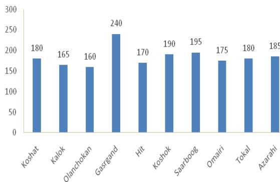
Figure (4): Rainfall Intensity for two days duration in Gasrgand District, flooded 19/1/2020 in Balochestan, Iran
