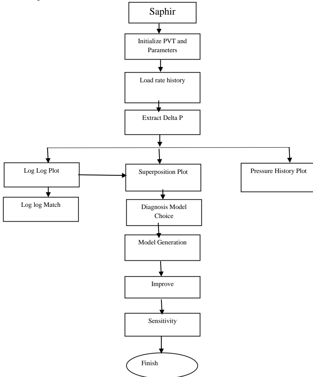
Fig. 2: Pressure Transient Analysis Workflow (Kappa Ecrin)
