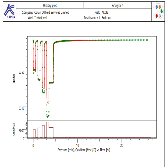
Fig. 27: History Plot Model Match
