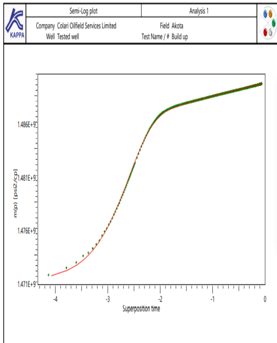
Fig.33: Semi-Log Plot Model Match
