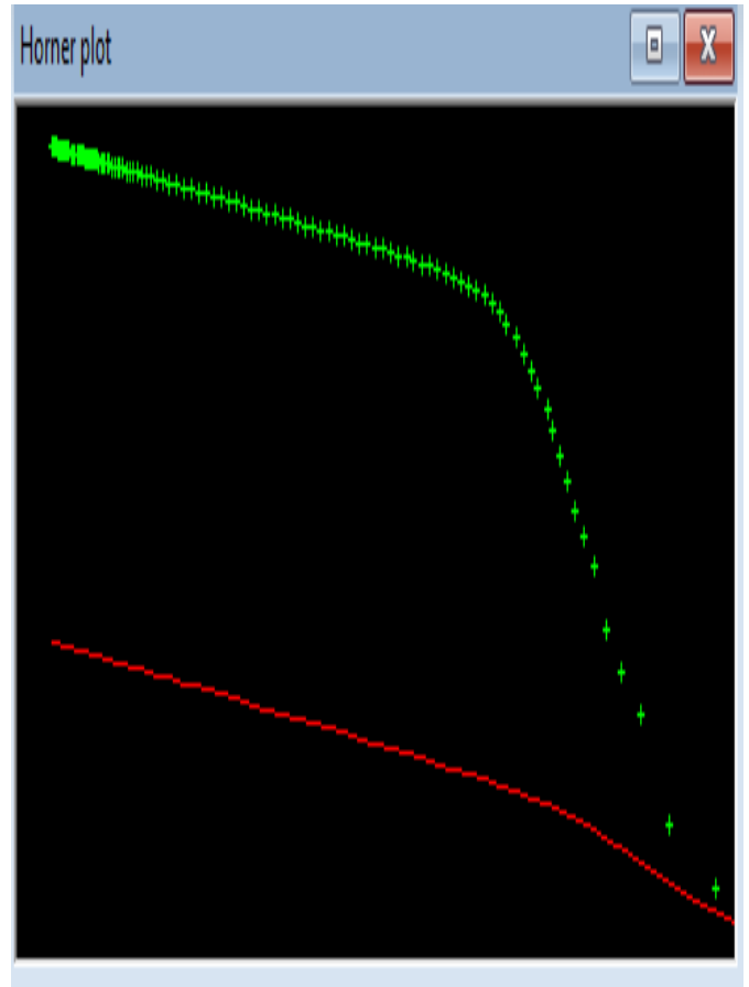
Fig. 17: Horner Plot Model Mismatch
