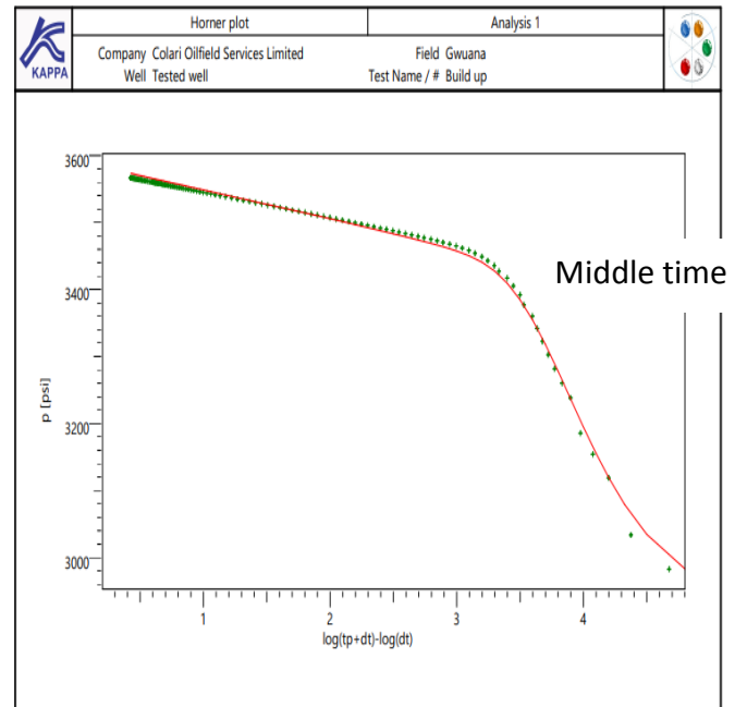
Fig. 18: Horner Plot Model Match
