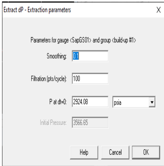
Fig. 11: Extract dialog 2
