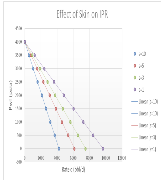
Fig.25: Effect of Skin on IPR
