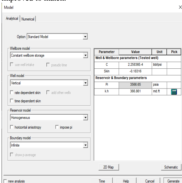
Fig.12: Model dialog
