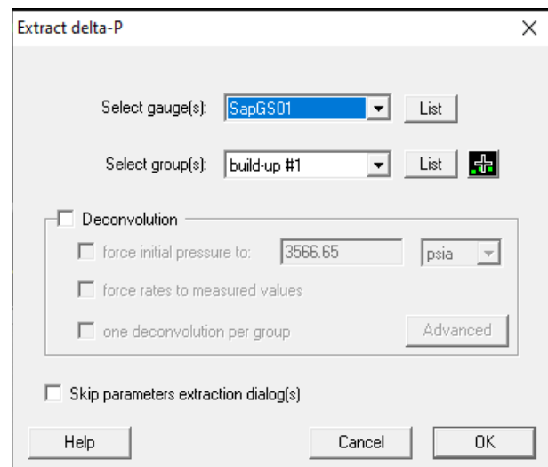
Fig. 10: Extract dialog 1
