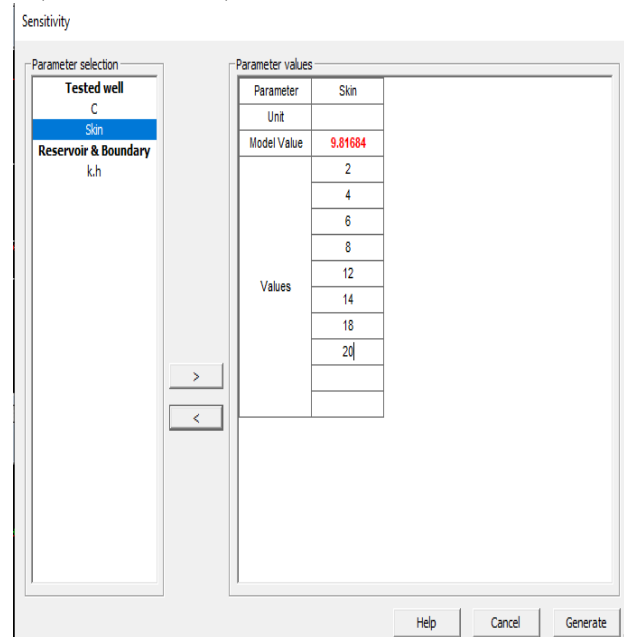
Fig. 14: Sensitivity Dialog
