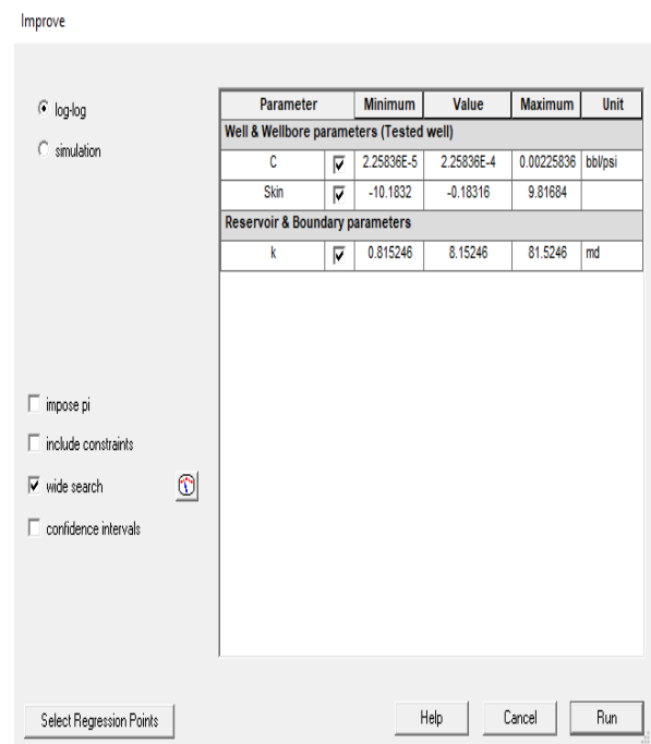
Fig.13: Improve Dialog
