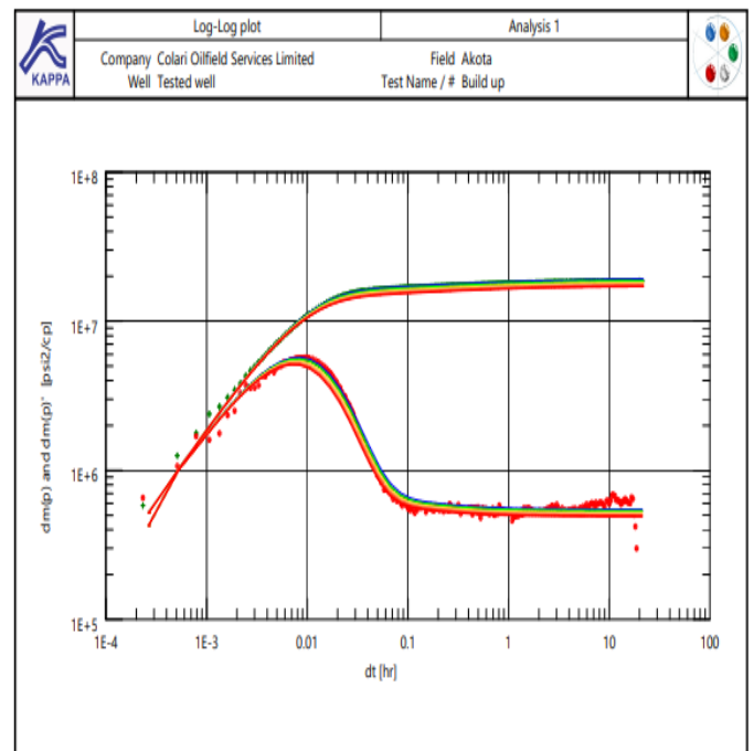
Fig. 36: Log-Log Plot - Permeability-Thickness Sensitivity Analysis
