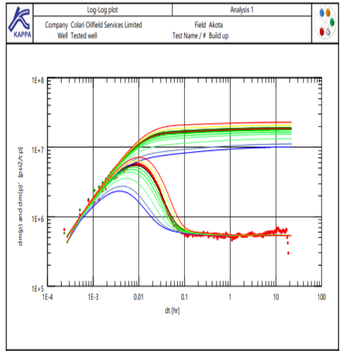
Fig. 35: Log-Log Plot - Skin Sensitivity Analysis
