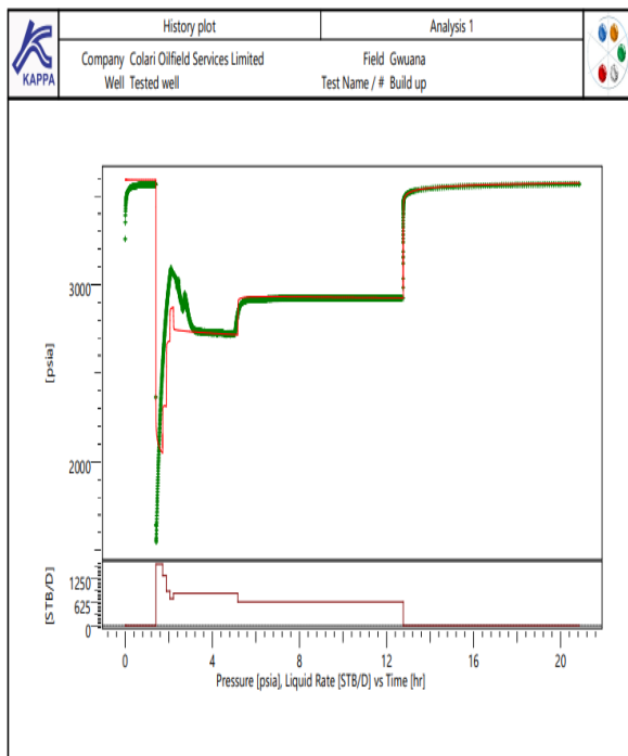
Fig. 16: History Plot Model Match
