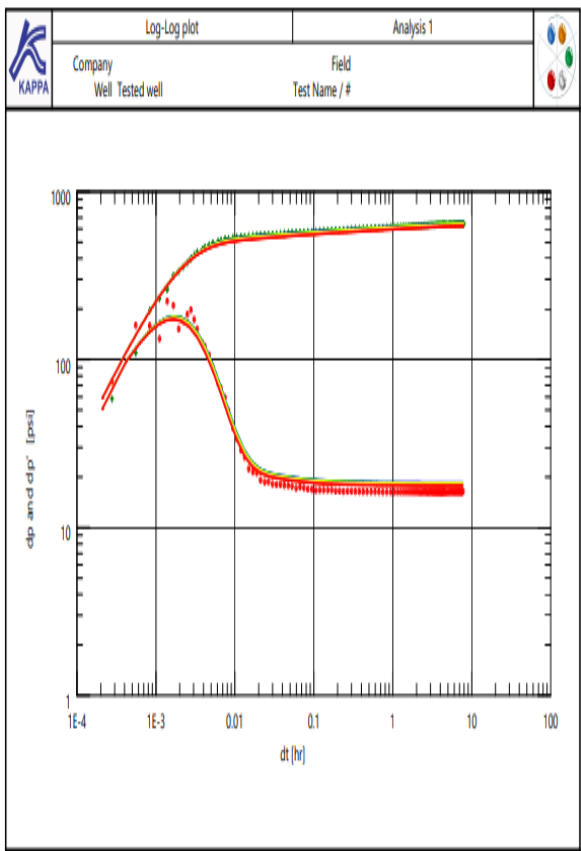
Fig. 24: Log-Log Plot – Permeability-Thickness Sensitivity Analysis
