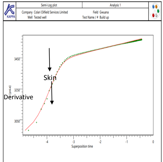
Fig. 22: Semi-Log Plot Model Match
