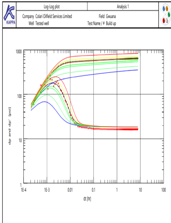
Fig. 23: Log-Log Plot - Skin Sensitivity Analysis
