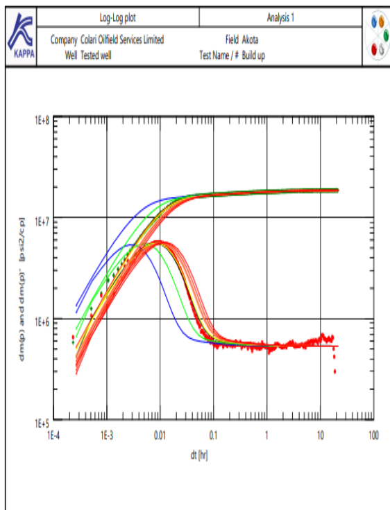
Fig.34: Log-Log Plot - Wellbore Storage Sensitivity Analysis
