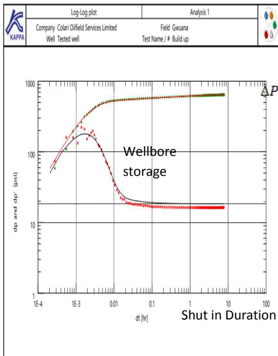
Fig. 20: Log-Log Plot Model Match
