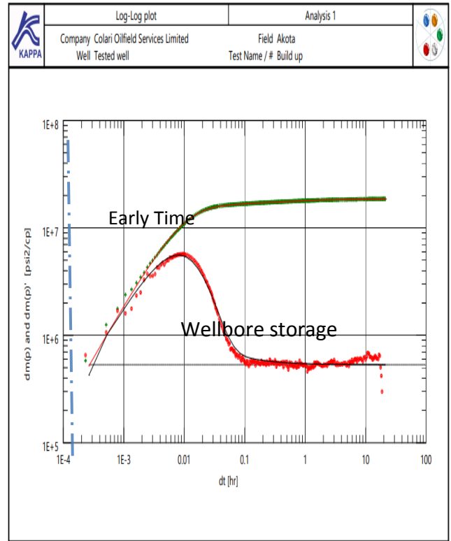
Fig. 31: Log-Log Plot Model Match
