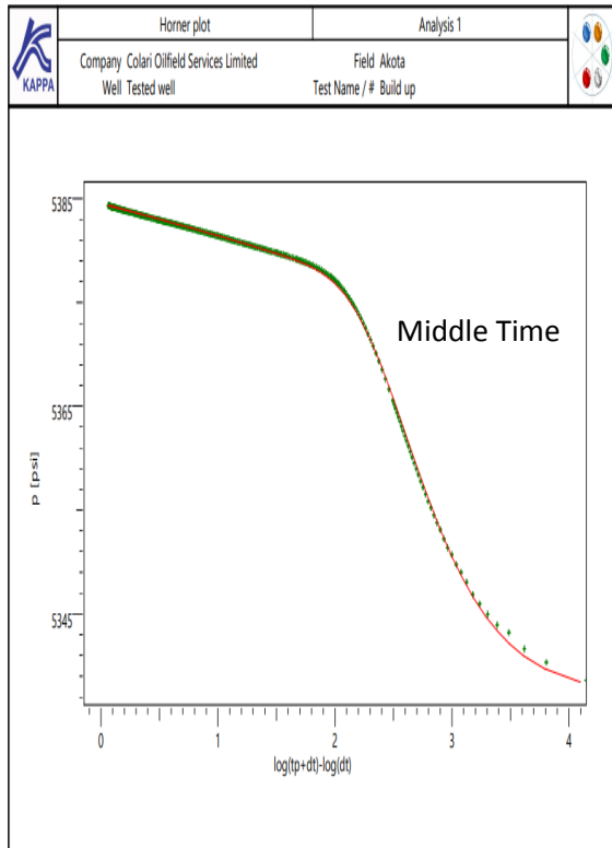
Fig. 29: Horner Plot Model Match
