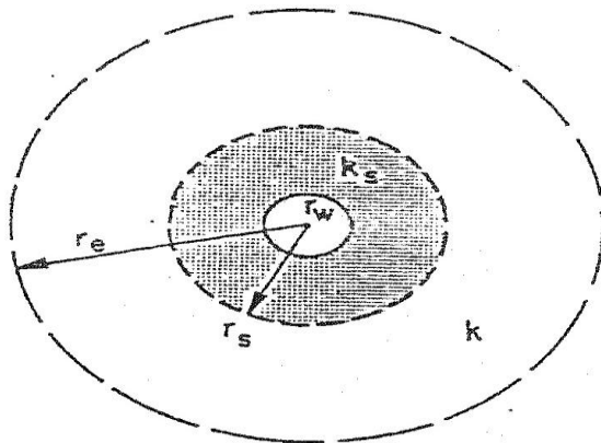
Fig. 1: A well with skin damage is illustrated in a diagram (Alhetari, 2017).
